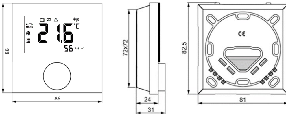
Fig. 1: Dimensions of Room Control Unit Display (in mm)
